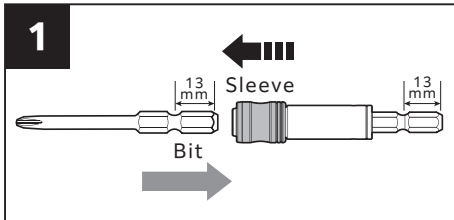
Slide the holder sleeve forward and attach the bit to the holder.
